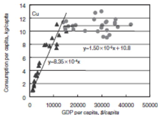
Fig. 4-11 Copper
