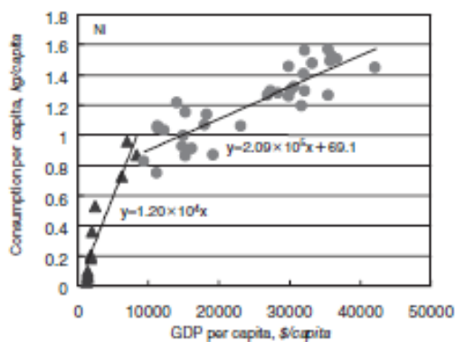
Fig. 4-2 Nickel
