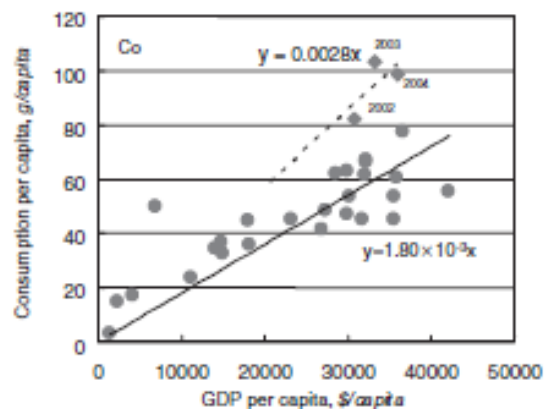
Fig. 4-19 Cobalt
