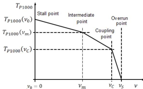
Figure 2 Generic torque ratio
