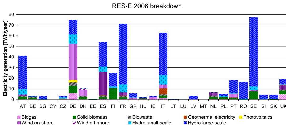
Source: Eurostat/Fraunhofer ISI: Electricity from renewable energy sources 2006 breakdown of normalised renewable electricity in 2006
